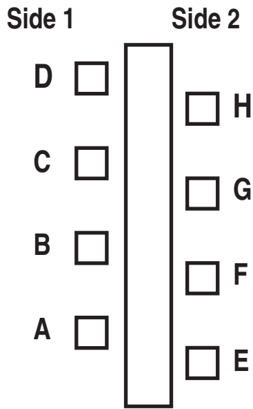
5 Way Standard "Fender" Type Open Frame Switch
