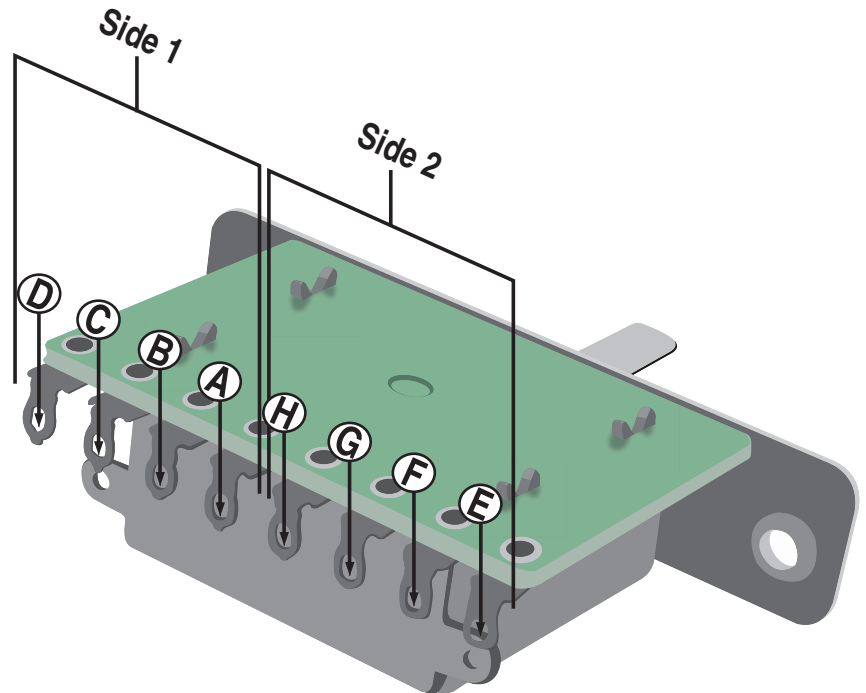
5 Way Inline "Carvin" Type Switch
